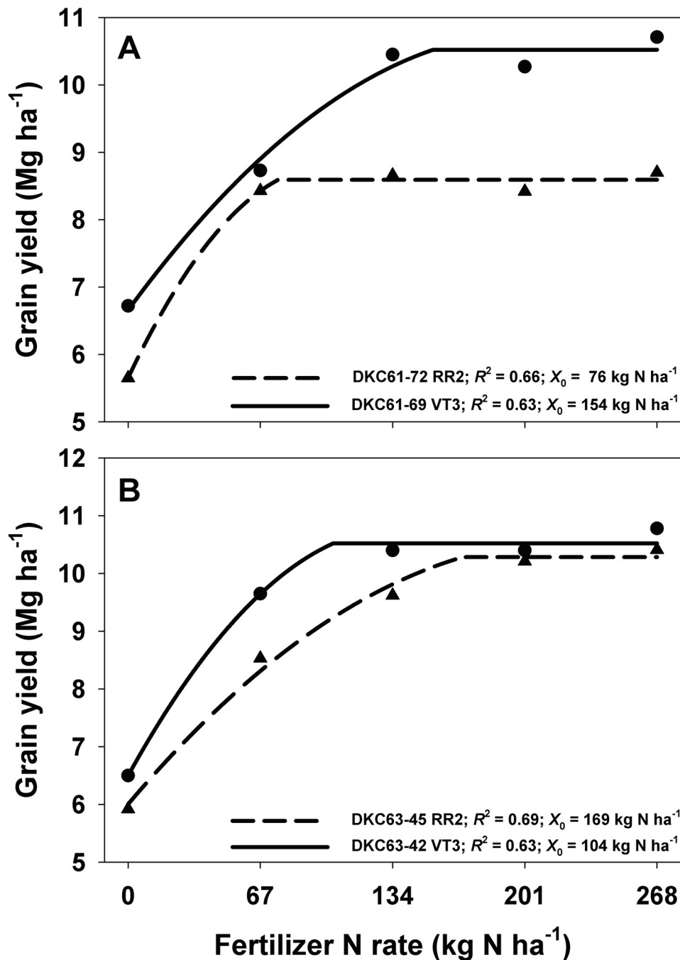
Figure 1. Response of grain yield to N for refuge (Roundup Ready Corn 2 [RR2]) and transgenic rootworm protected (YieldGard VT Triple [VT3]) hybrids. The hybrids included a 111 d relative maturity (RM) pair (A) (DKC61-72 RR2 and DKC61-69 VT3) and a 113 d RM pair (B) (DKC63-45 RR2 and DKC63-42 VT3). Curves were fitted using quadratic with plateau regression functions with data combined across both years of the study. All regression models were significant at P \leq 0.001 . Predicted maximum grain yields were 8.6 and 10.5 Mg ha -1 for DKC61-72 and DKC61-69 and 10.3 and 10.5 Mg ha -1 for DKC63-45 and DKC63-42. Individual points represent the grain yield means for each hybrid \times N rate treatment combination averaged across both years of the study.
